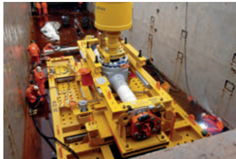
Subsea Riser Positioning
